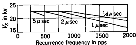
FIG. 8-10.— V_s as a function of recurrence frequency.
